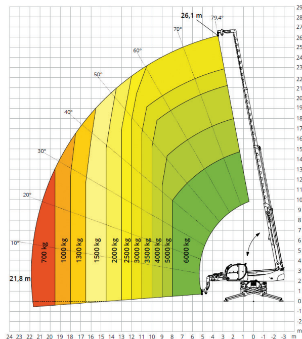
Lasthaken 6,0 to
